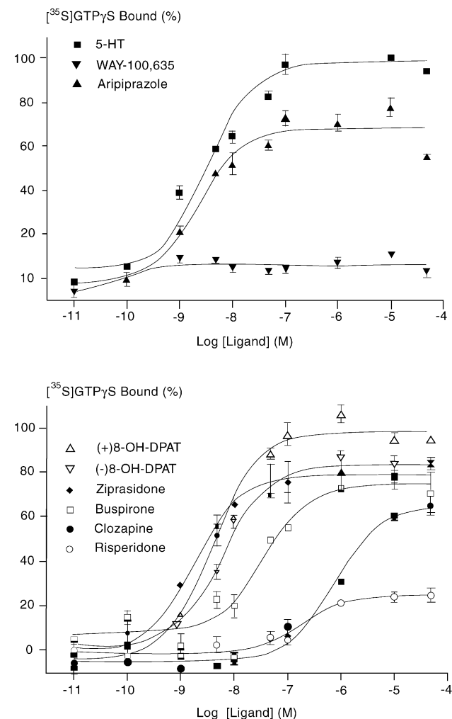
Fig. 1. Drug effects upon basal [^3\text{S}]\text{GTP}\gamma\text{S} binding to CHO cell membranes expressing the h5-HT 1A receptor. All data points are means \pm S.E.M. of triplicate determinations from a single representative experiment and are expressed as a percentage of the stimulatory effect of 10 \mu\text{M} 5-HT on basal [^3\text{S}]\text{GTP}\gamma\text{S} binding.
